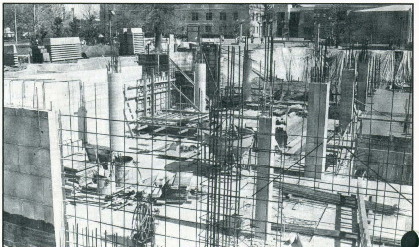
This area will contain the subplaza classrooms (view toward the east)
