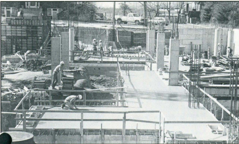
Concrete finishing work in the subplaza classroom area (view toward the west)
